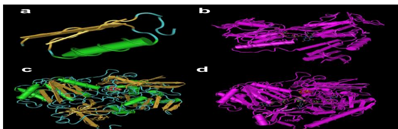
Figure 4. 3D structure modeling of nitrite reductase. a nasD predicted by SWISS MODEL, b nasD most similar protein predicted by NCBI blastp, c nasE predicted by SWISS MODEL, d nasE most similar protein predicted by NCBI blastp
